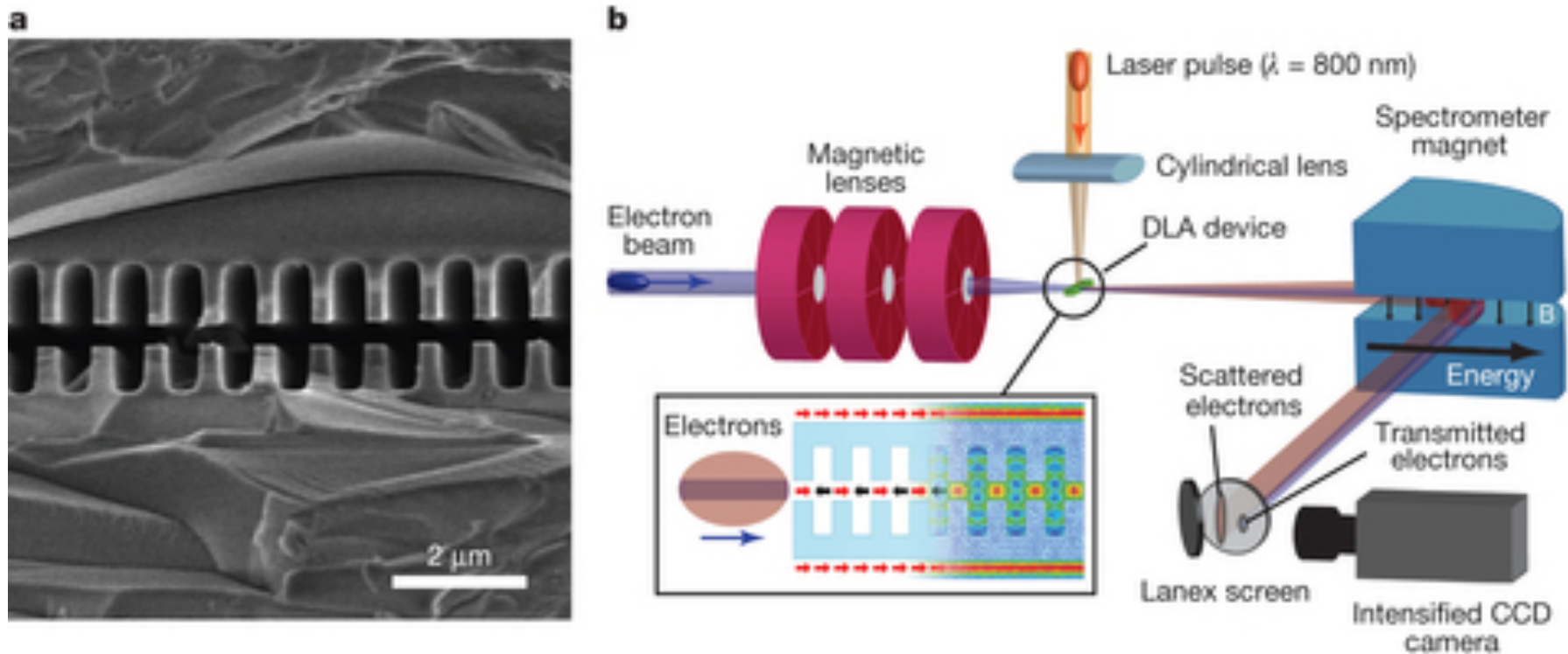
Scanning electron microscope image of the longitudinal cross-section of a DLA structure fabricated as depicted in Extended Data Fig. 1a. Scale bar, 2 \mu\text{m} . b, Experimental set-up.
