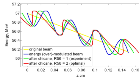
S. Antipov et al., PRL 111, 134802 (2013) Microbunching @ BNL ATF
