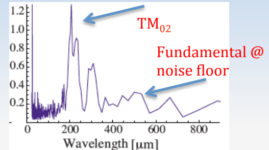
G. Andonian et al., APL 98, 202901 (2011) Selective mode excitation @BNL ATF
