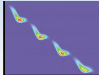
G. Andonian et al., APL 98, 202901 (2011) Selective mode excitation @BNL ATF
