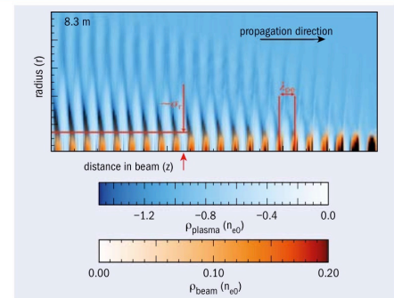
Fig. 1. Simulation of a self-modulated proton bunch resonantly driving plasma wakefields sustained by the plasma-density perturbation. The plasma density is shown increasing from white to blue and the proton density increasing from yellow to dark red.
