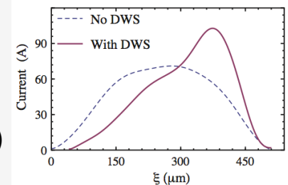
G. Andonian et al., PRL 118, 054802, (2017) Ramped beam @ BNL ATF
