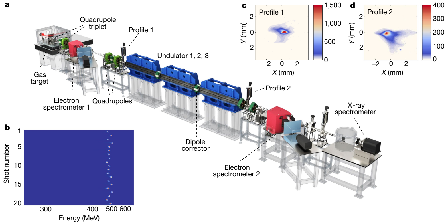
Fig.1|Schematic layout of LWFA-based free electron laser experiment. a , Undulator beamline with a total length of approximately 12 m from the gas target for the LWFA to the X-ray spectrometer. b , Typical spectra of electron
