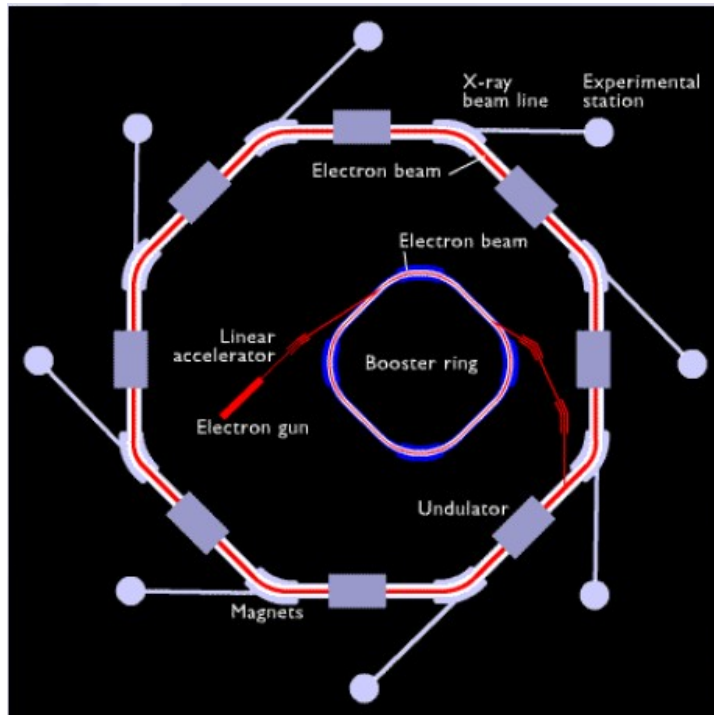
undulator
