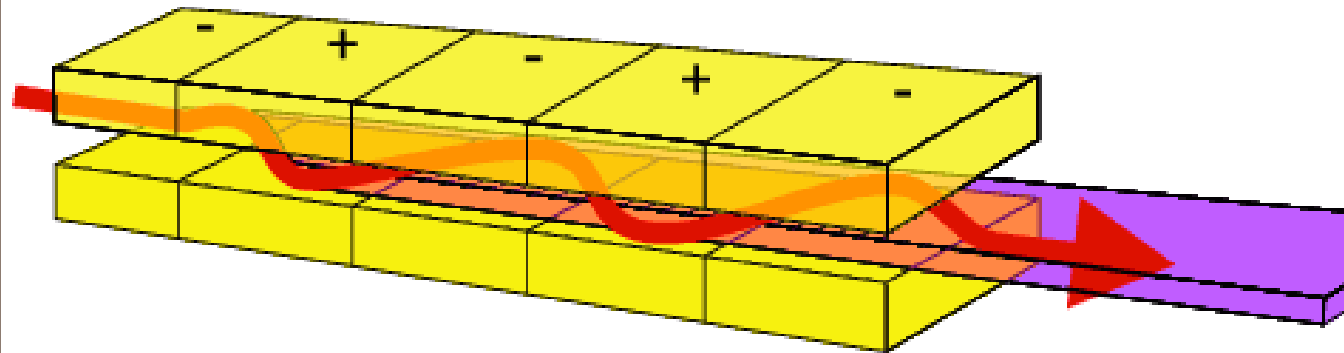
undulator
