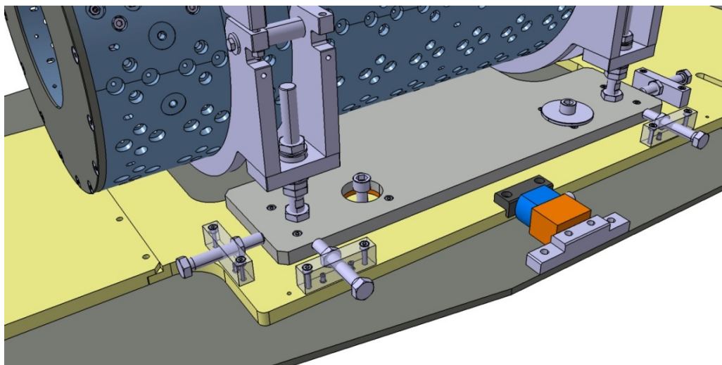
Magnet support and tuning system
