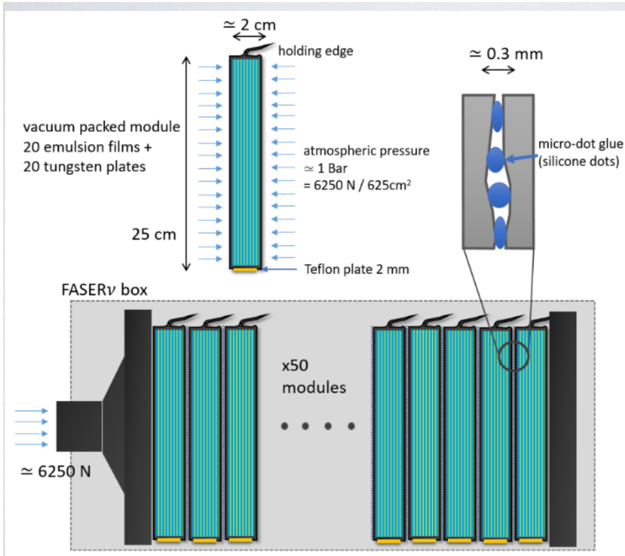
Vacuum-packed module
