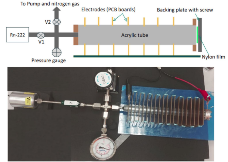
FIG. 2. Top: diagram of the radon daughter deposition chamber showing the components. Bottom: photo of the assembled system.
