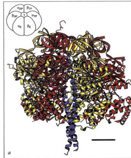
F1-ATPase, 1994 https://www.nature.com/articles/370621a0
