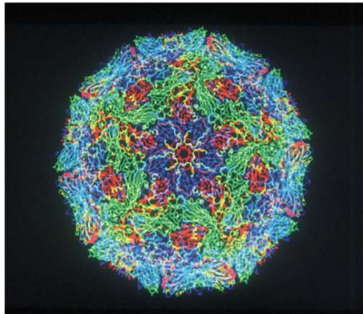
FMDV Structure, 1989 https://www.nature.com/articles/337709a0
