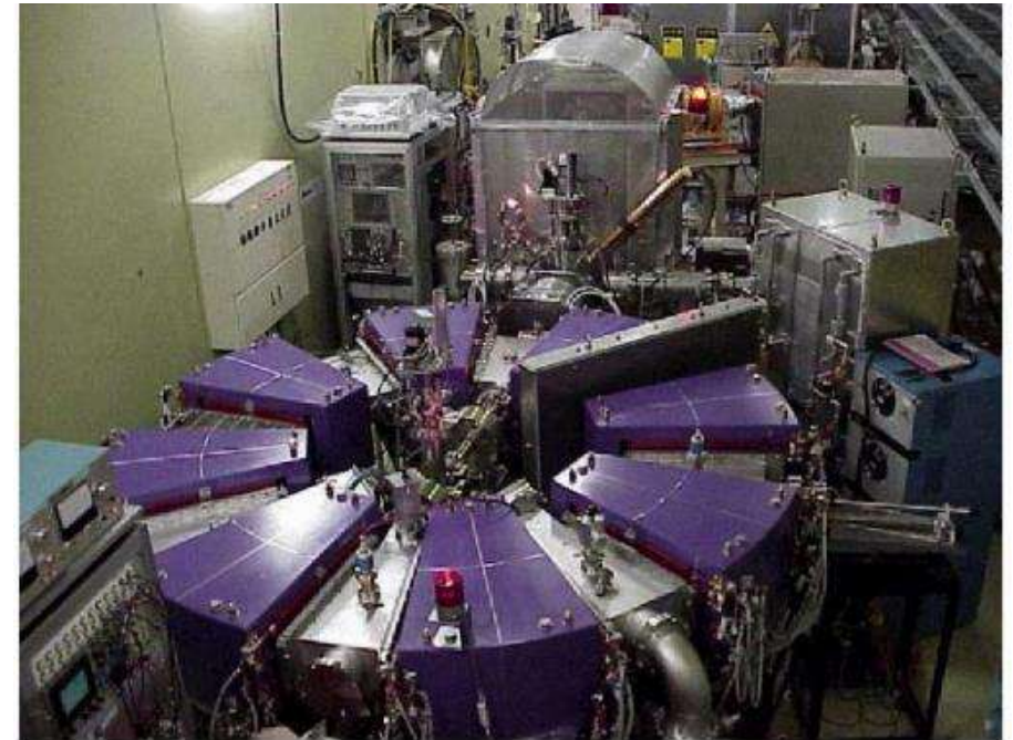
KEK, 2000. First proton FFAG
